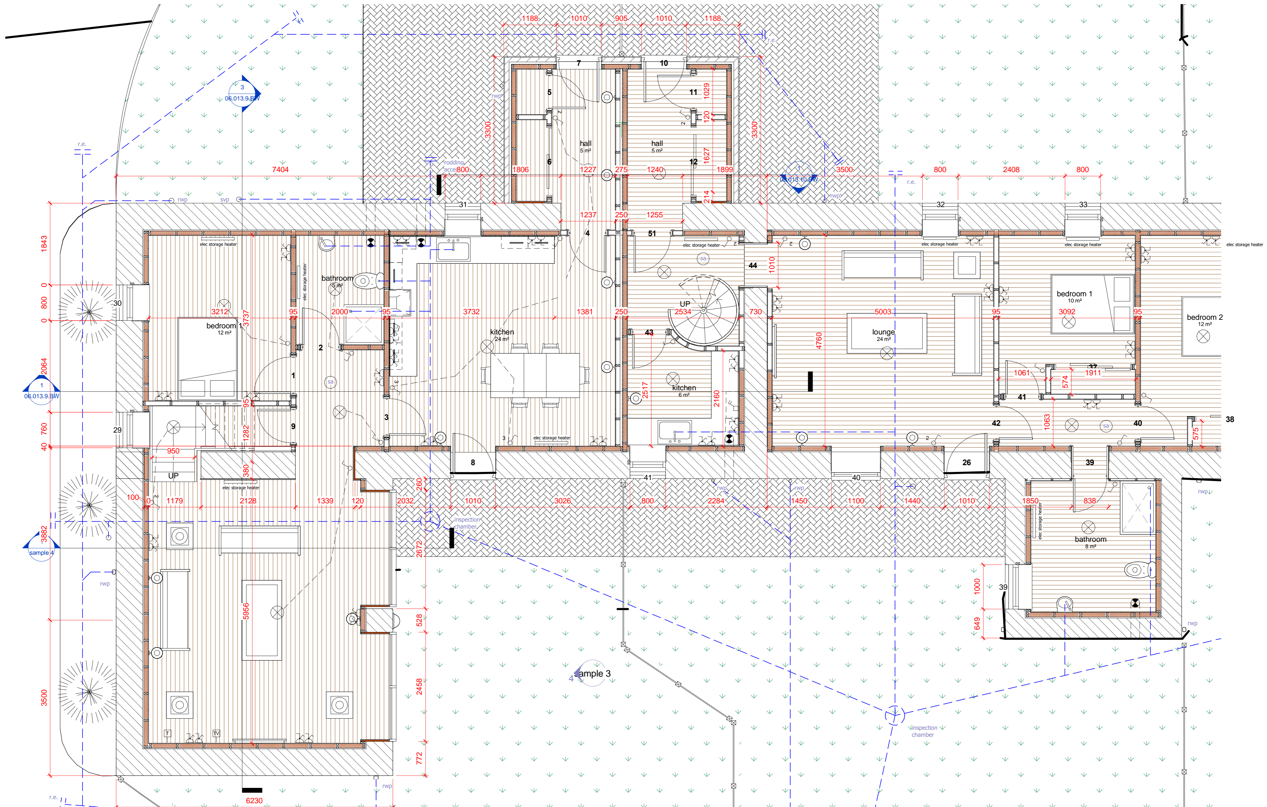
1 1. ground floor 1 : 50
